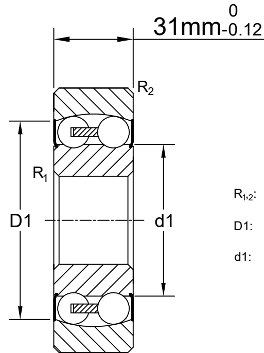
LILY BEARING
